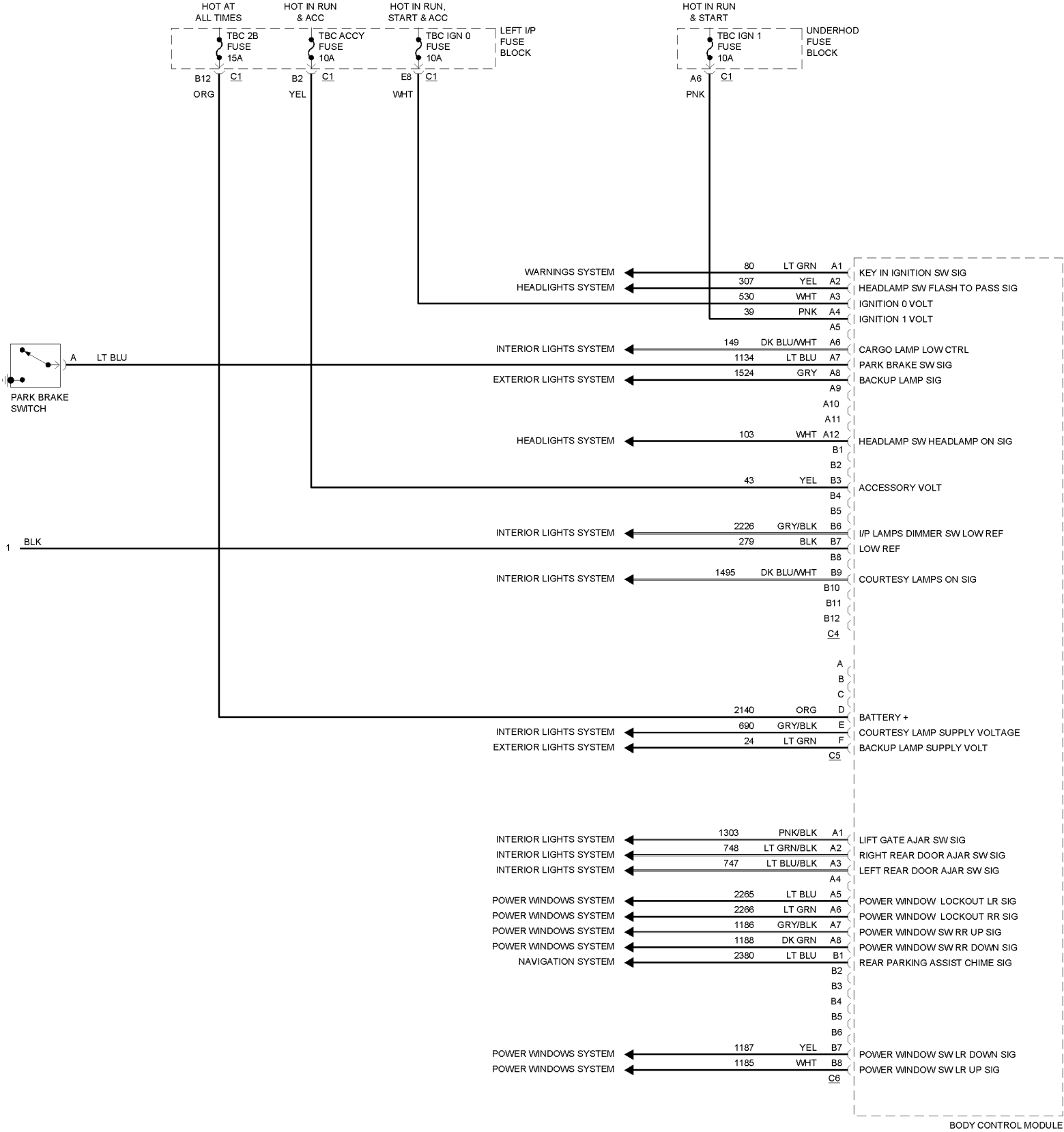
BODY CONTROL MODULE
